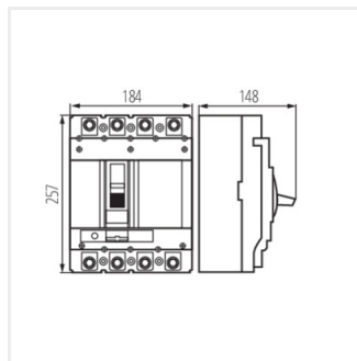
KMCCB-RT-400A-4P-H
