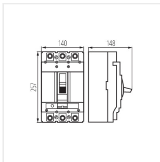
KMCCB-RT-400A
